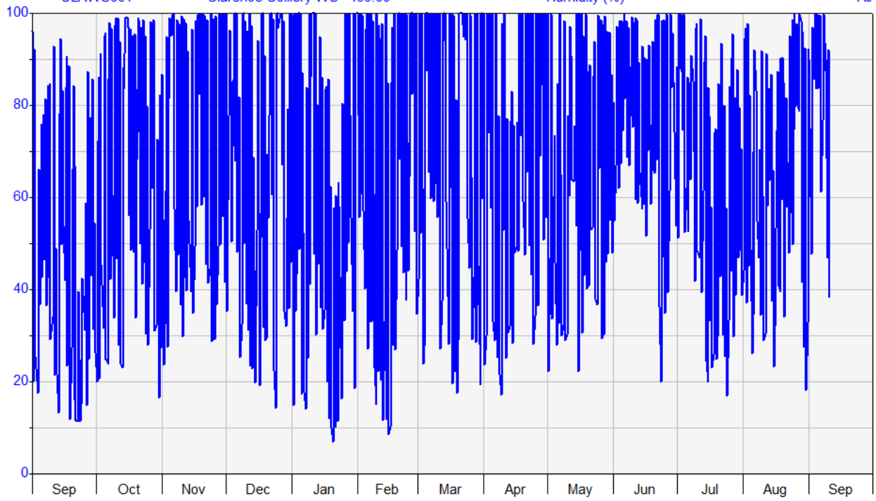
Figure 7 – 12 Monthly Relative humidity
